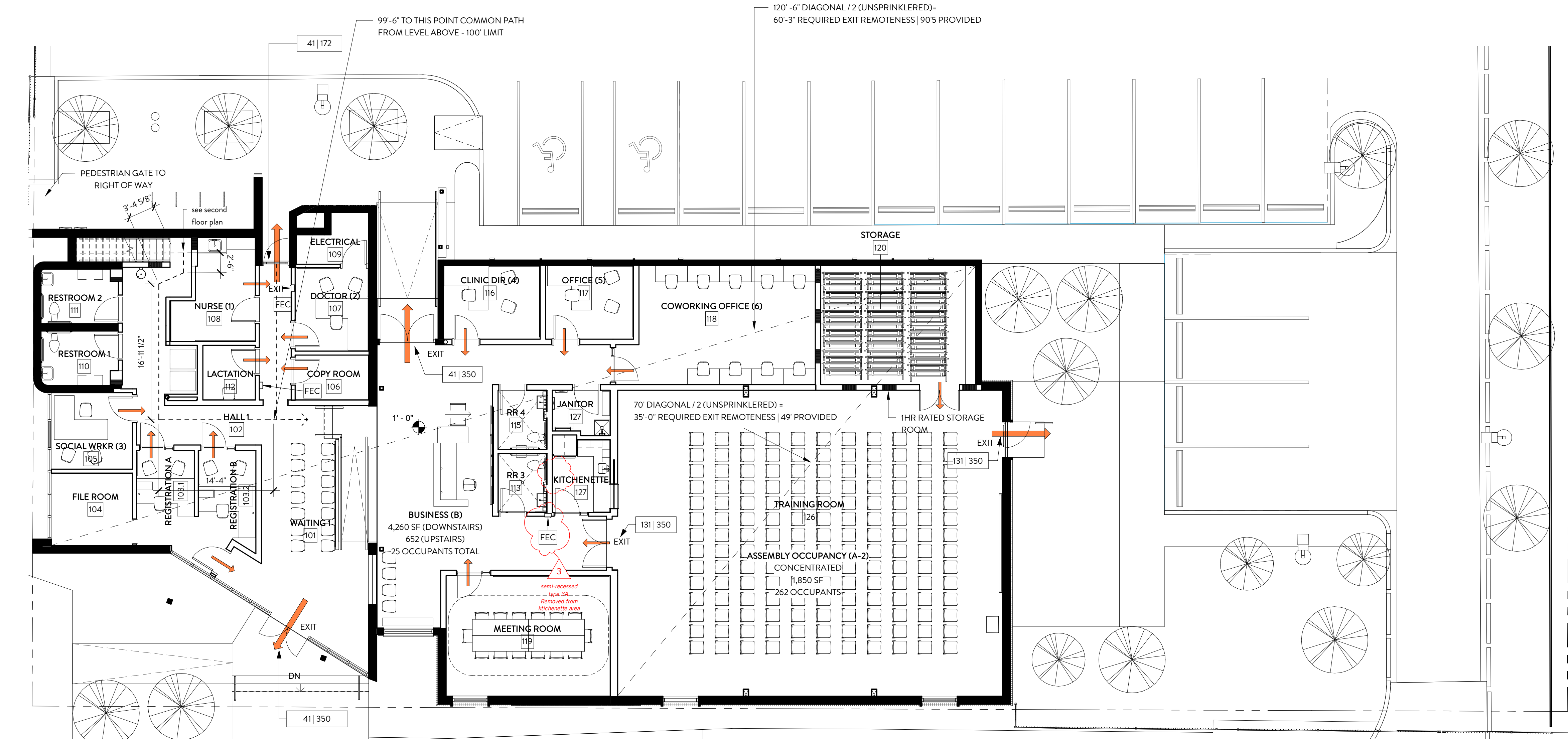
2 MEZZANINE - AREA PLAN - LIFE SAFETY A003 1/8" = 1'-0"
