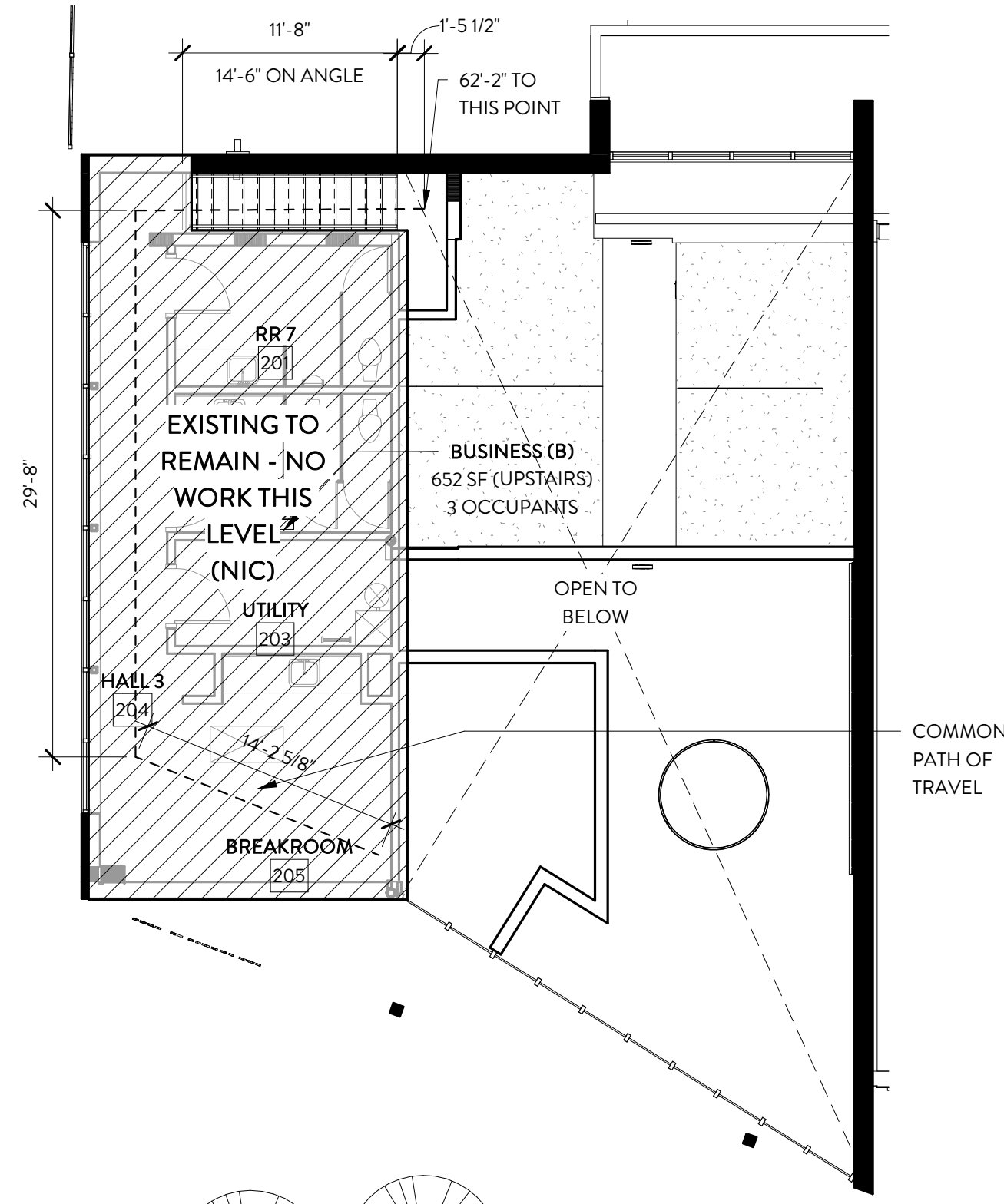
2 MEZZANINE - AREA PLAN - LIFE SAFETY A003 1/8" = 1'-0"
